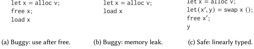
Fig. 2. Memory safety.
